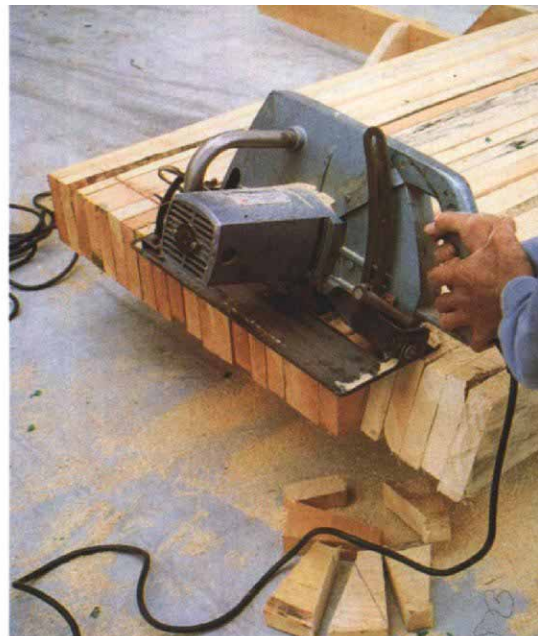
To save time, ridges can be gang-cut with a 16-in. beam saw (photo right). Though these saws won't cut all the way through anything wider than a 2x4 at a 4-in-12 pitch, where necessary each cut can be completed using a standard circular saw. For these finish cuts, the kerfs guide the saw. The only layout required is a single chalkline across the top edge of the rafters. An alternate method is to use a Linear Link saw (photo left), a Skil worm-drive saw fitted with a bar and chain.
