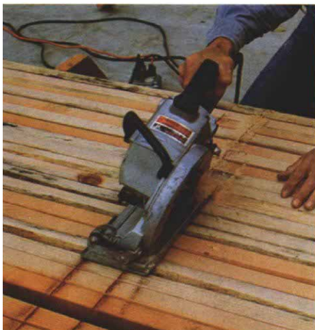
One method for gang-cutting birds' mouths is to cut the heels with a worm-drive saw (photo left) and the seats with a worm-drive saw fitted with a swing table, an accessory base that adjusts from -5° to 68° (photo right). By equipping a saw with a universal dado kit (photo above), birds' mouths up to 3/4 in. wide can be plowed out in a single pass.
