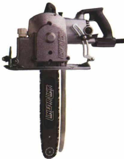
To save time, ridges can be gang-cut with a 16-in. beam saw (photo right). Though these saws won't cut all the way through anything wider than a 2x4 at a 4-in-12 pitch, where necessary each cut can be completed using a standard circular saw. For these finish cuts, the kerfs guide the saw. The only layout required is a single chalkline across the top edge of the rafters. An alternate method is to use a Linear Link saw (photo left), a Skil worm-drive saw fitted with a bar and chain.
